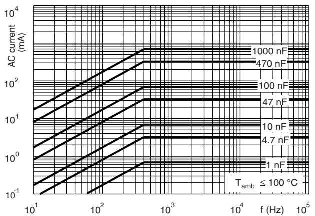
Max. RMS voltage and AC current (sinewave)
