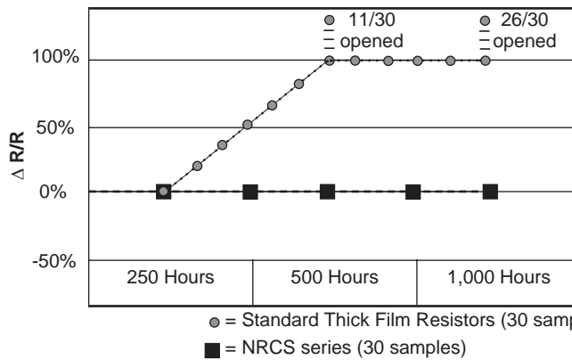
Typical Performance* (After immersions in cutting fluid with 0.5% Sulfur content)
