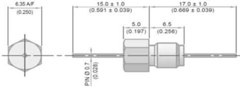
2BA Thread
